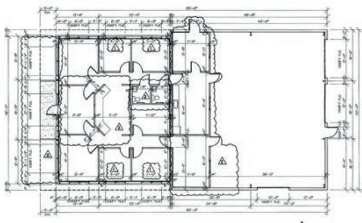
Floor Plan 6281
